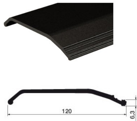
PROFILO IN PVC
