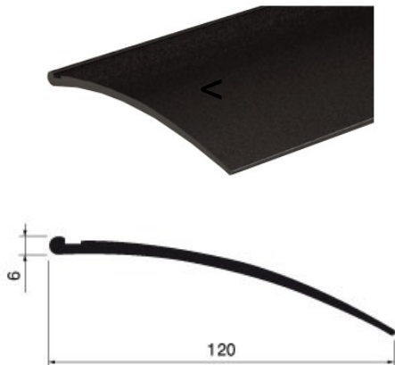
PROFILO IN PVC
