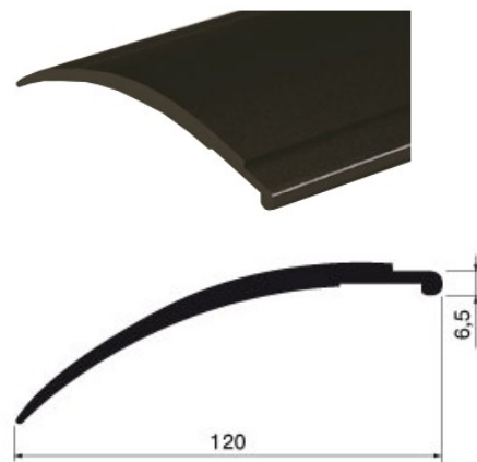
PROFILO IN PVC
